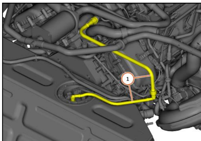
Layout overview - Fuel hoses to be replaced (1) (extract from SCB 14 K 001 WI)
