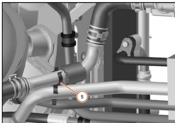
Layout overview - Install clip assembly (5) and move pipe protector
